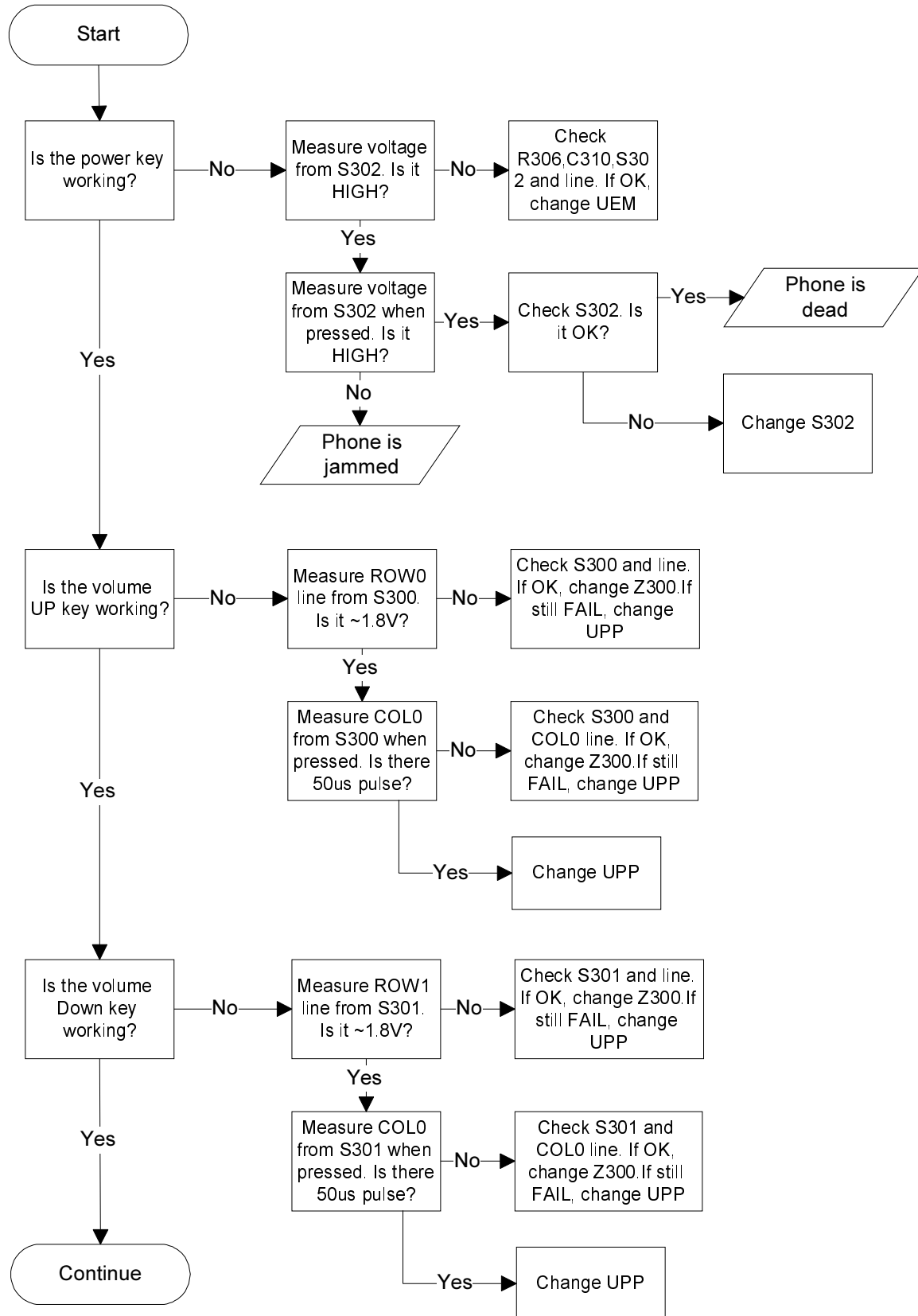
Figure 25: Keypad troubleshooting 1
